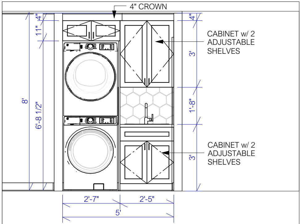
Ⓑ LAUNDRY DETAIL B 3/8 in = 1 ft
