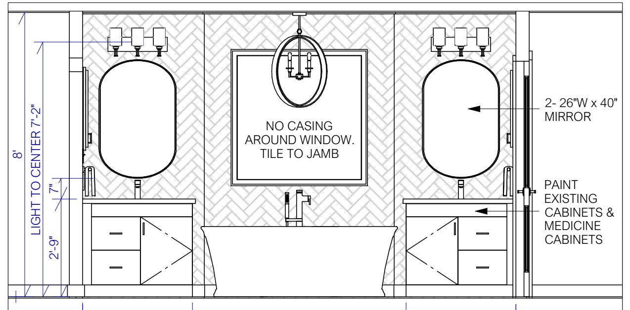
Ⓐ ENSUITE WALL DETAIL - A 3/8 in = 1 ft
