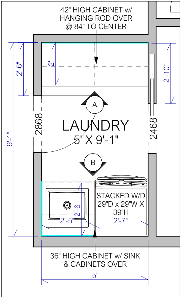
Ⓒ LAUNDRY ROOM DETAIL 3/8 in = 1 ft
