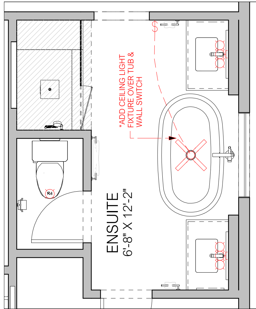
○ ELECTRICAL PLAN 3/8 in = 1 ft
