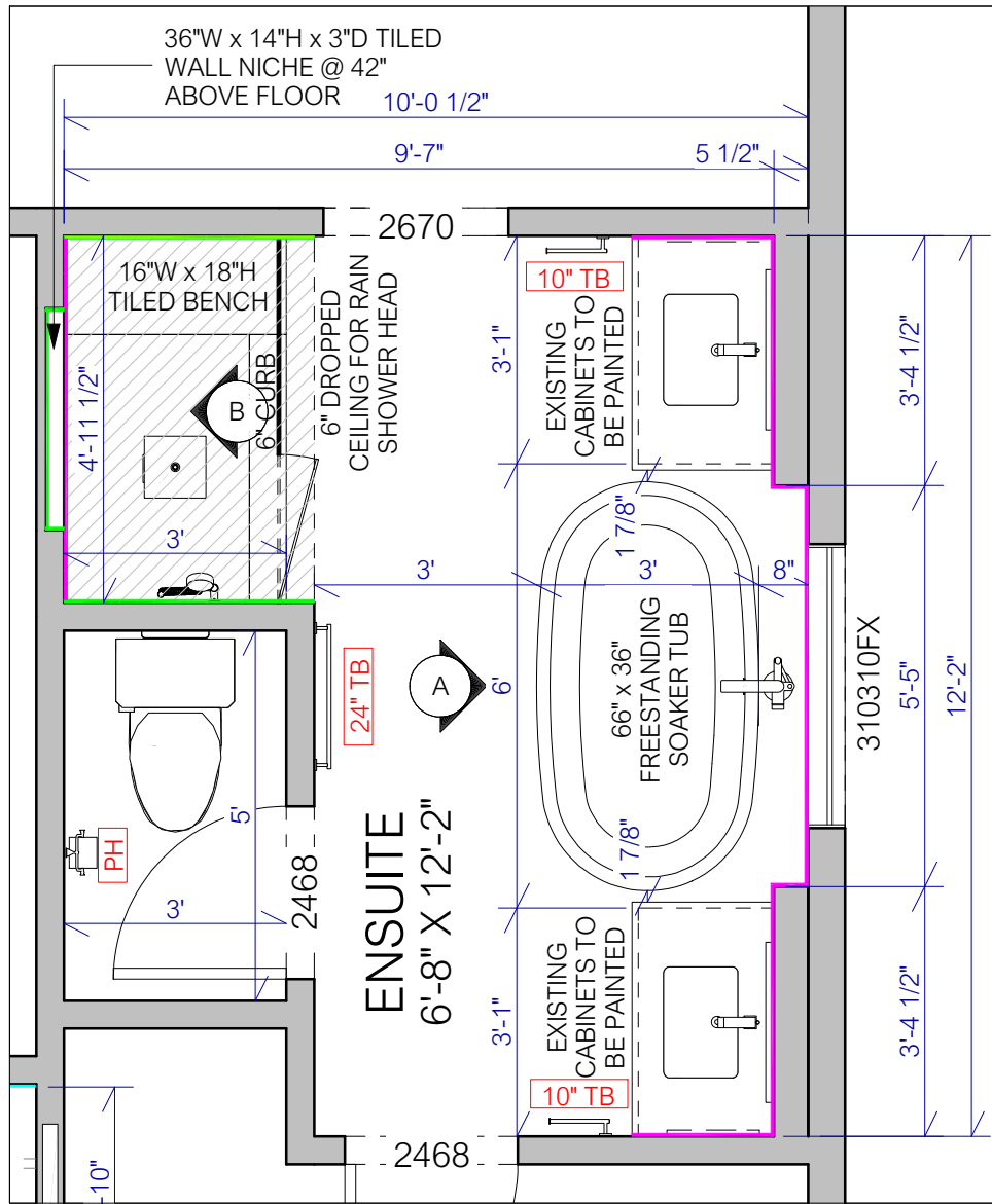
○ ENSUITE PLAN 3/8 in = 1 ft
