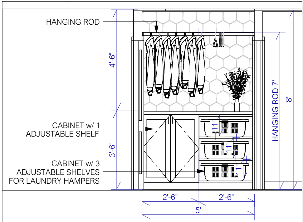
Ⓐ LAUNDRY DETAIL A 3/8 in = 1 ft
