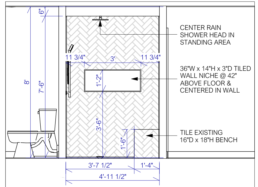
Ⓑ SHOWER NICHE DETAIL - B 3/8 in = 1 ft
